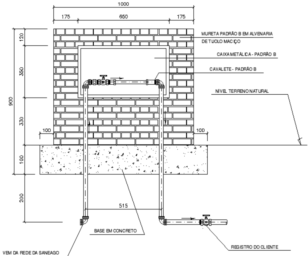
VISTA FRONTAL
