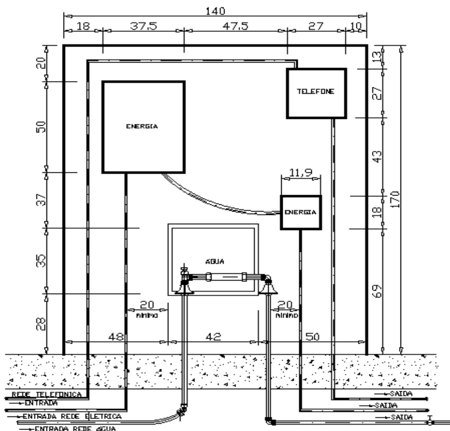
VISTA FRONTAL
