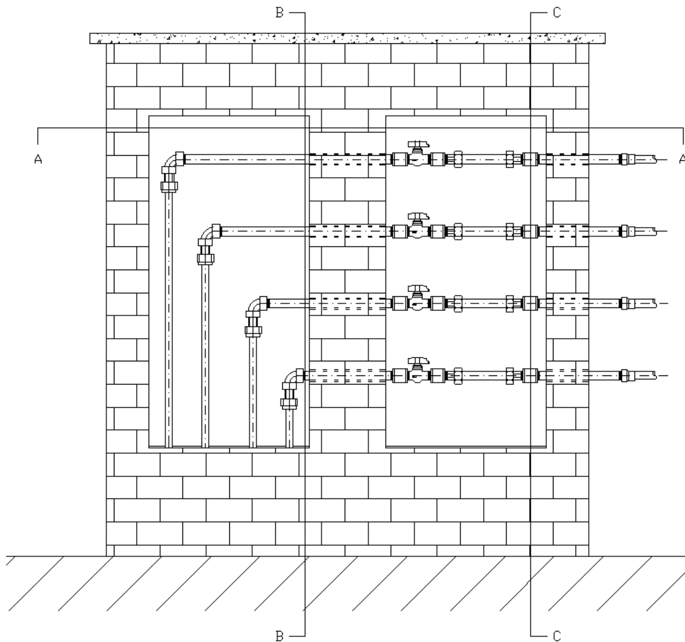
VISTA FRONTAL
