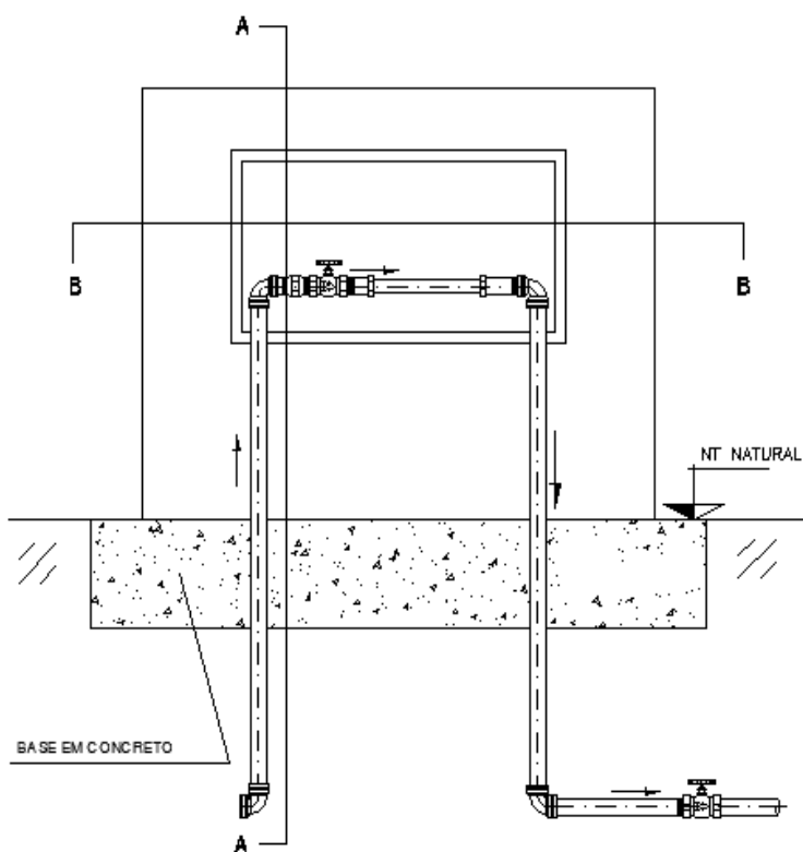
VISTA FRONTAL
