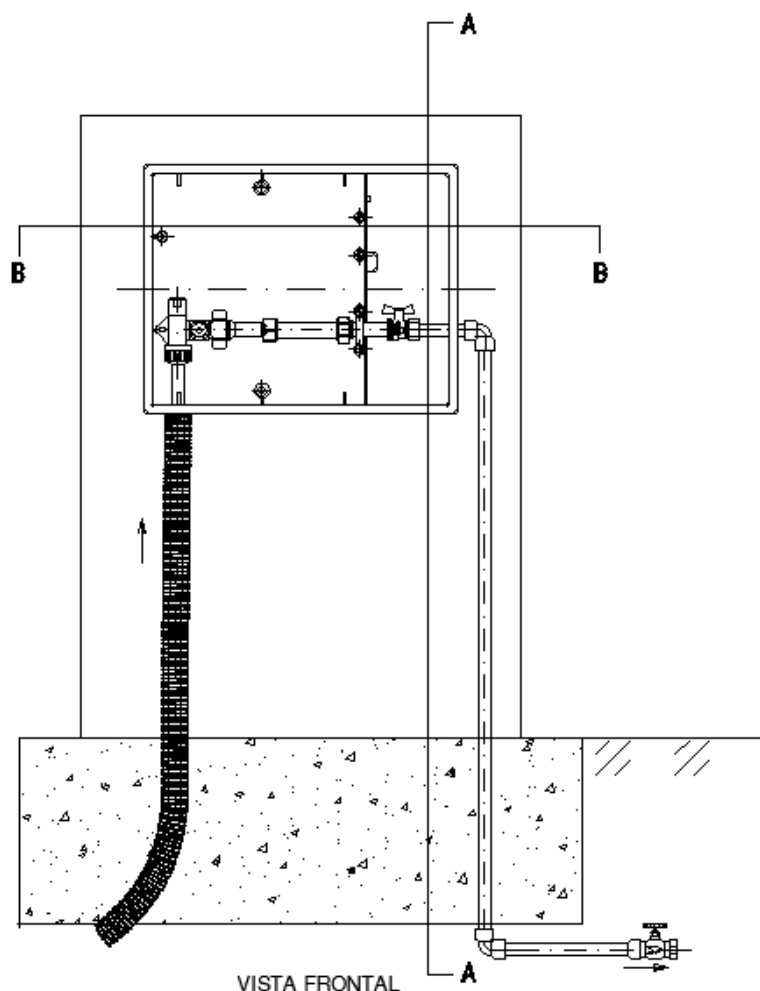
VISTA FRONTAL
