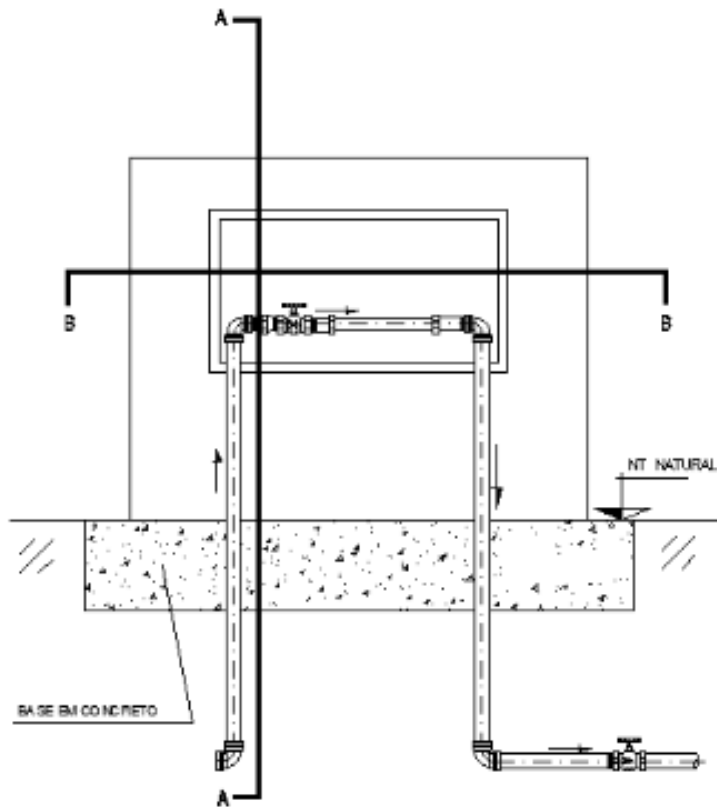
VISTA FRONTAL
